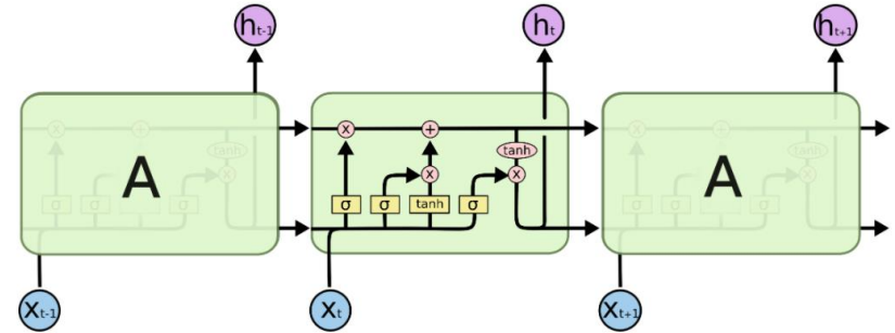
Long short-term memory
